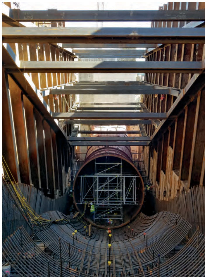
Fall 2017 steel liner installation into penstock
